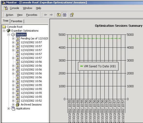
Sessions Summary The Sessions view contains a list of all optimizations that have been completed to date , allowing administrators to gauge how much Virtual Memory is saved per user session .
